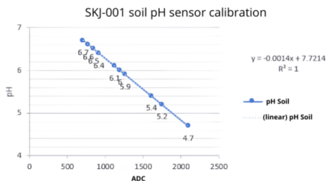
Figure 16. Calibration Graph for Soil pH Sensor SKJ-001
