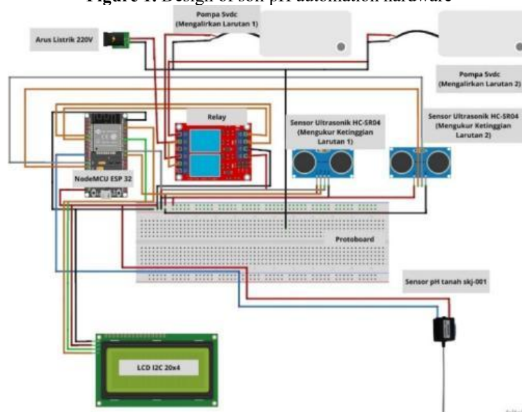
Figure 2. Schematic diagram of soil pH automation circuit
