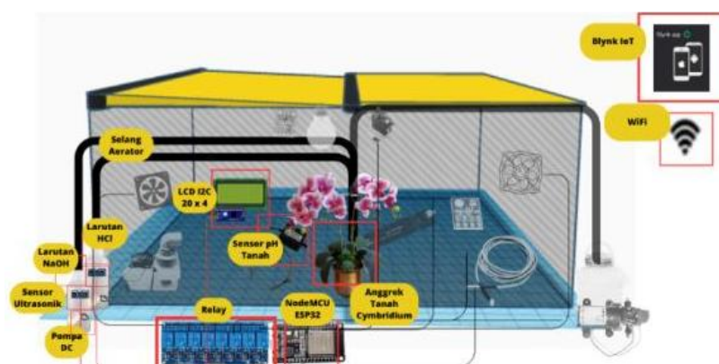
Figure 1. Design of soil pH automation hardware
