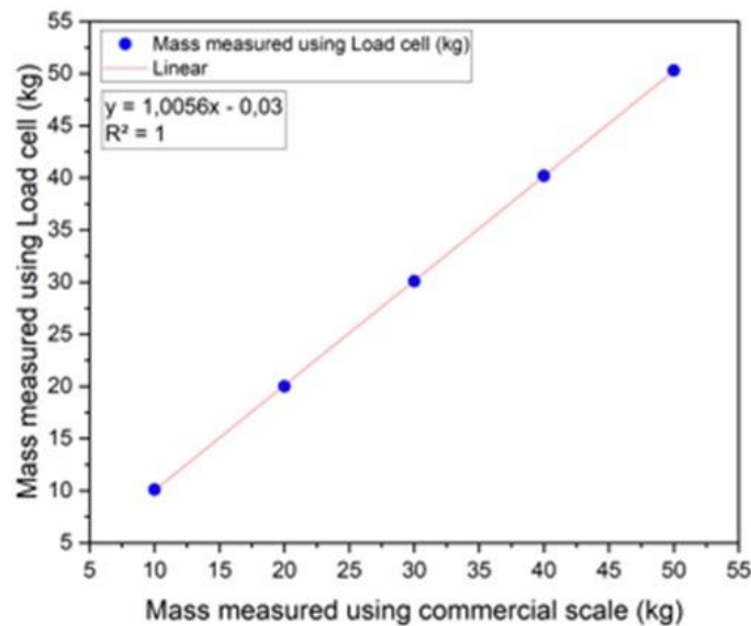
Figure 6 Load cell characterization.
